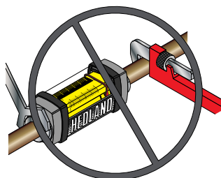
Figure 2: Installing the meter
