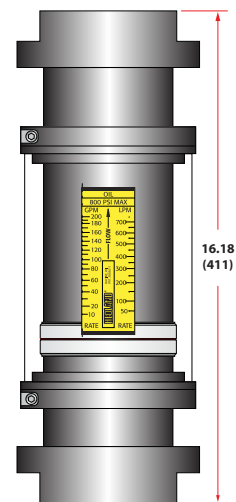
Figure 11: 3 inch; C61 Flange Inches (mm)
