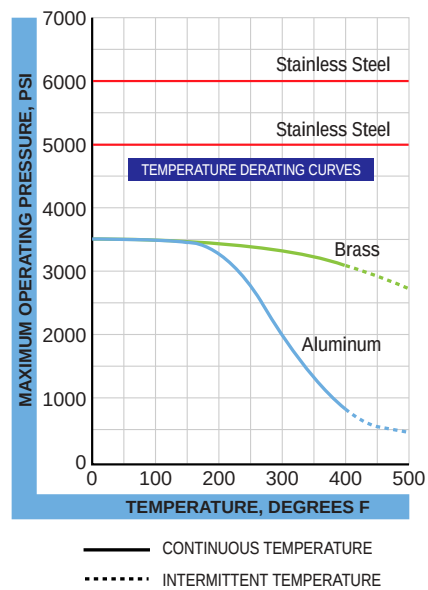
Figure 8: Pressure vs temperature
