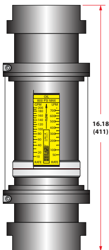
Figure 10: 3 inch; SAE, NPTF, BSPP Inches (mm)
