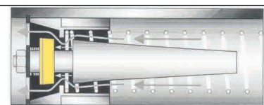
Reverse flow by-pass
