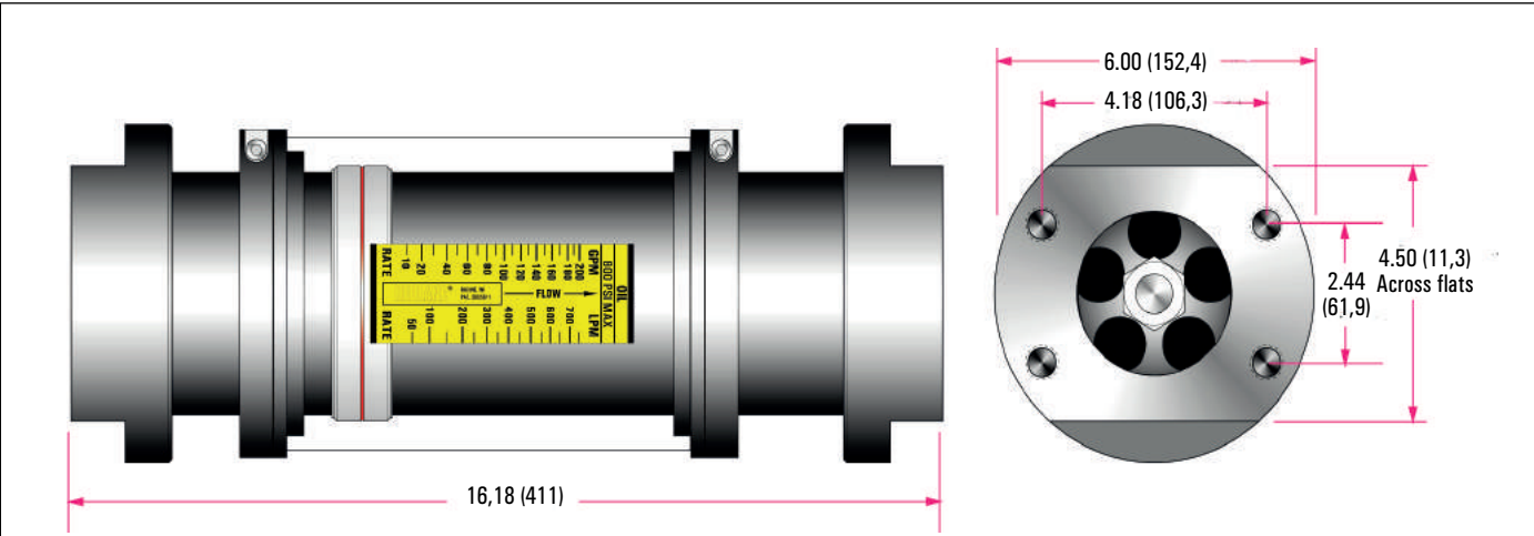
3 inch; C61 flange - Inches (mm)
