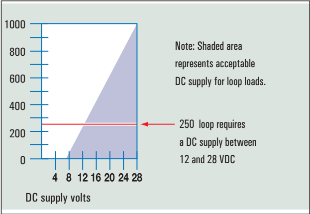
Figure 1: Load limitations (4-20 mA output only)
