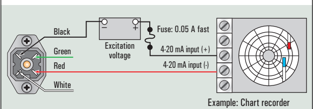
Schematic 3: 4-20 mA connection using target external power supply
