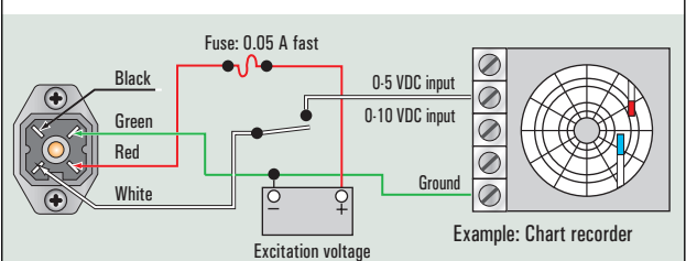
Schematic 4: 0-5 Vdc or 0-10 Vdc connection using target external power supply
