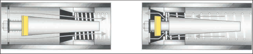
Normal flow direction
