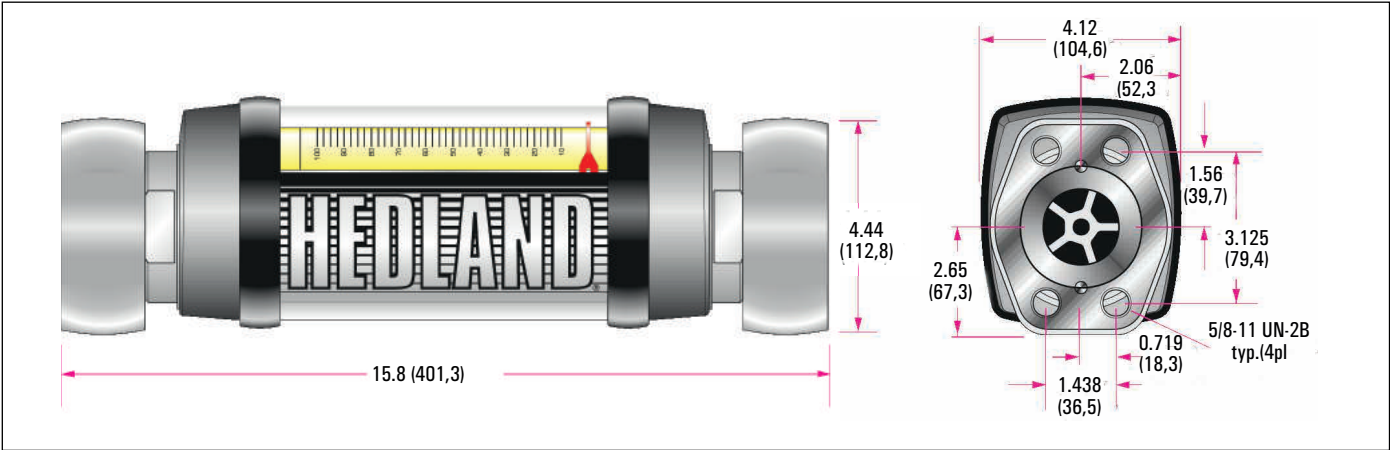
1½ inch; C62 flange - Inches (mm)
